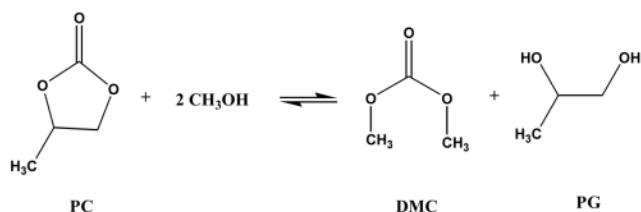
Scheme 1. Synthesis of DMC from PC and methanol.
